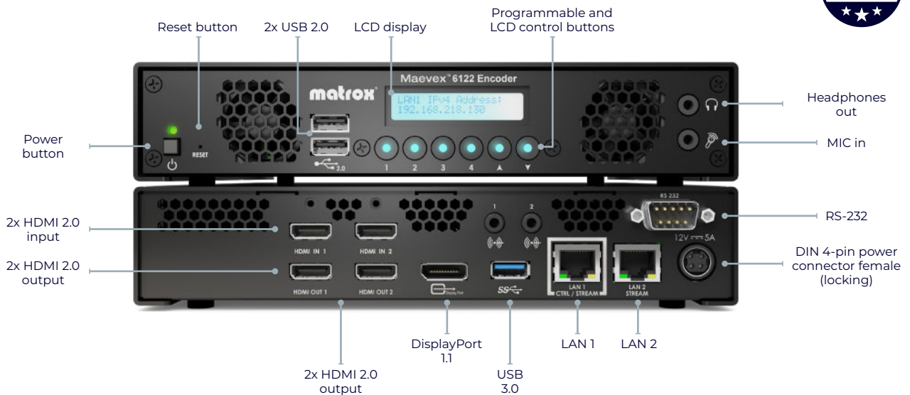
Matrox MaeveX 6122 dual 4K encoder (front/back view)
